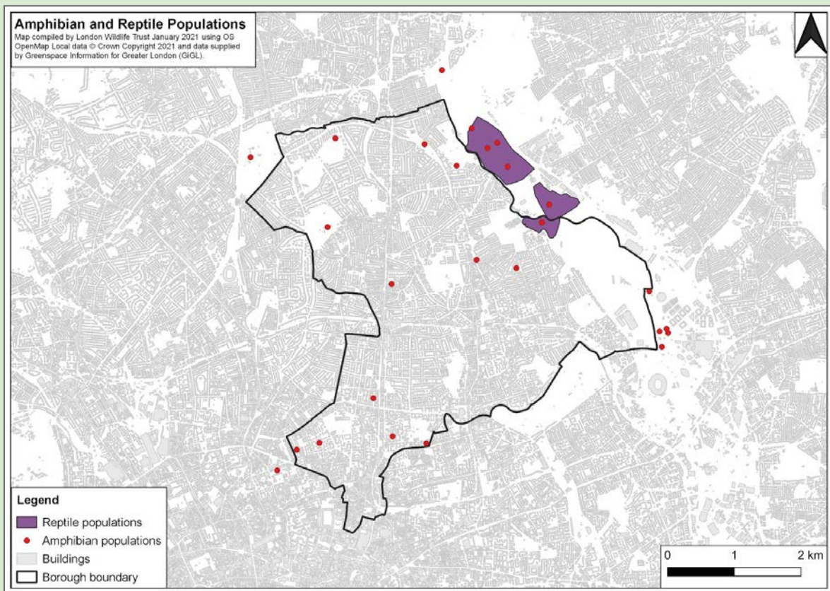
Figure 4: Amphibian and Reptile populations.
